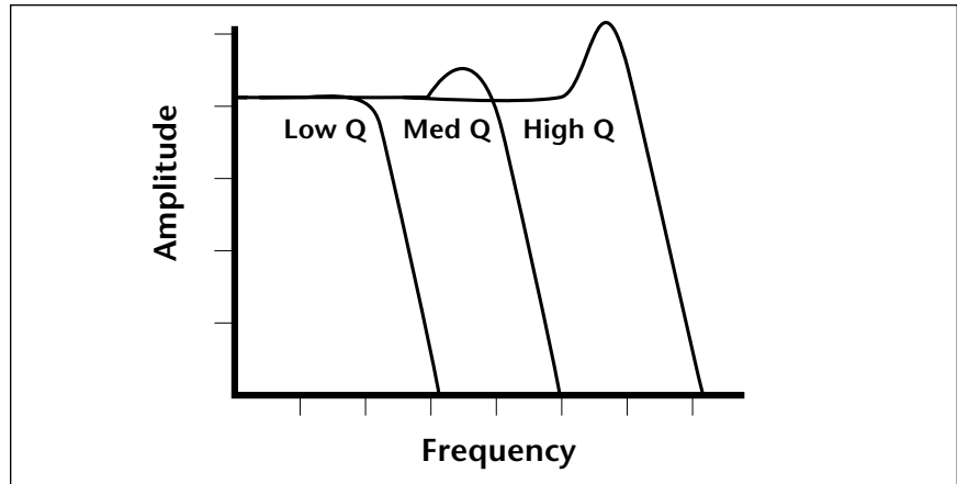
Turning up the “Q” emphasizes the frequencies around the cutoff point.
